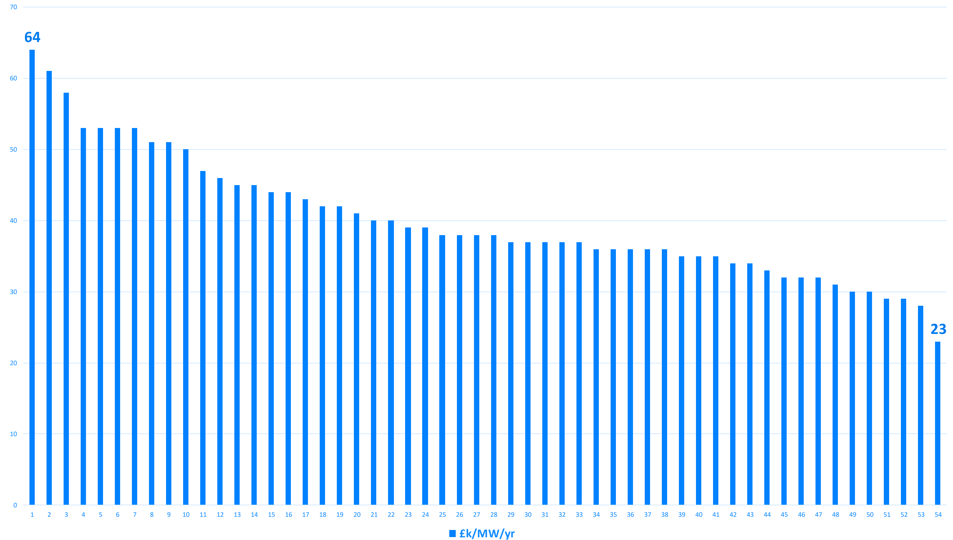
asset performance of selected BESS in UK (June 12, 2023 - June 12, 2024)
